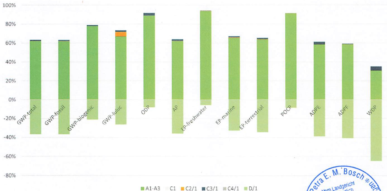
Relative contributions of the various life cycle phases of the blaugelb Insulation Panel EPS (100 % material recycling)
